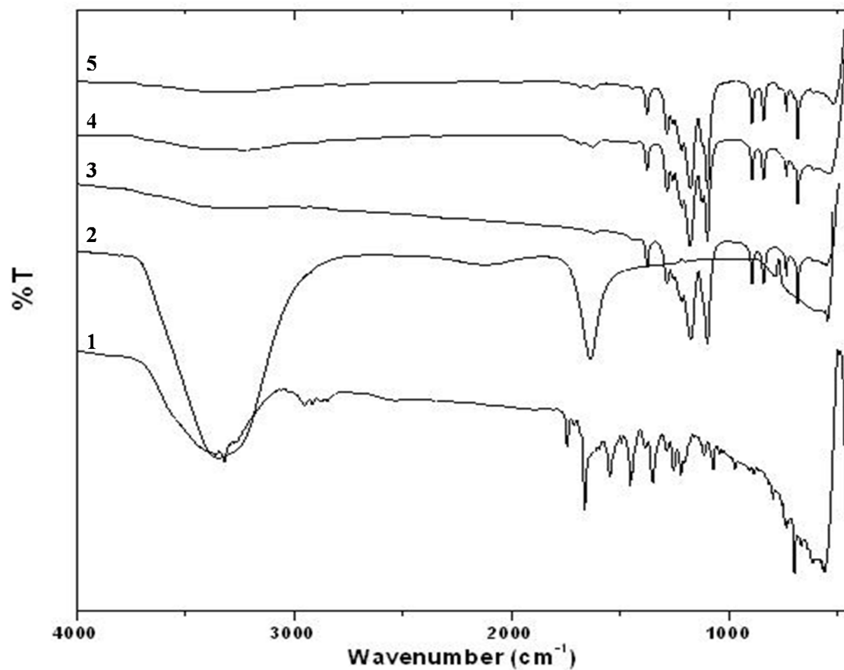
FTIR Spectra of solid FF dipeptide, FF nanotubes and FF dipeptide at various dilutions in HFIP solvent. [1] Solid FF dipeptide; [2] FF nanotubes; [3] FF in HFIP (10%w/v); [4] FF in HFIP (5% w/v); [5] FF in HFIP (2.5% w/v)
