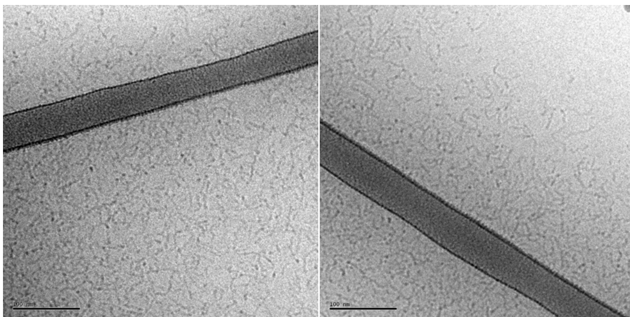
Figure 1a. Additional cryo-TEM images showing the worm-like micelles.
