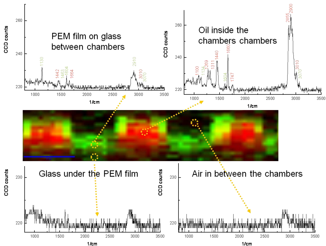
Figure 1. Raman spectra taken from different parts of the PEM chambers filled with sunflower oil. Bands marked with green correspond to PEMs; bands marked with red correspond to sunflower oil.
