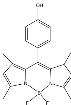
Figure S5. Structure of Bodipy.
