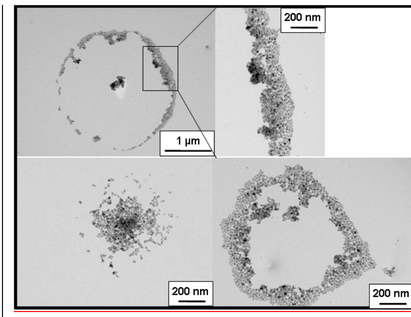
Figure S1. TEM micrographs of vesicles synthesized with DDAB and showing the encapsulation of large magnetic nanoparticles (LMNPs) ( d = 13.3 \text{ nm} ; \sigma = 0.34 ) using REV process.
