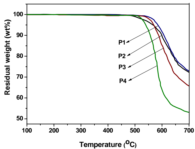
Fig. S1 TGA curves of the four polyimides.
