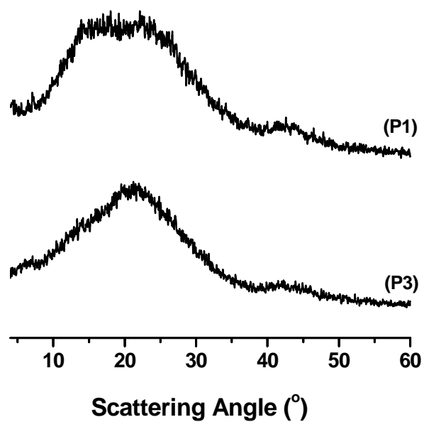
Fig. S2 WAXD patterns of polyimide networks
