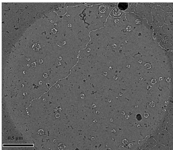
Figure 1 Cryo-EM images of nano-spheres and worm-like micelles in a solution composed of 8 mg/ml P123 in DMF and 29 wt% H 2 O, starting from a water solution containing P123 and then adding DMF. The bar corresponds to 500 nm.
