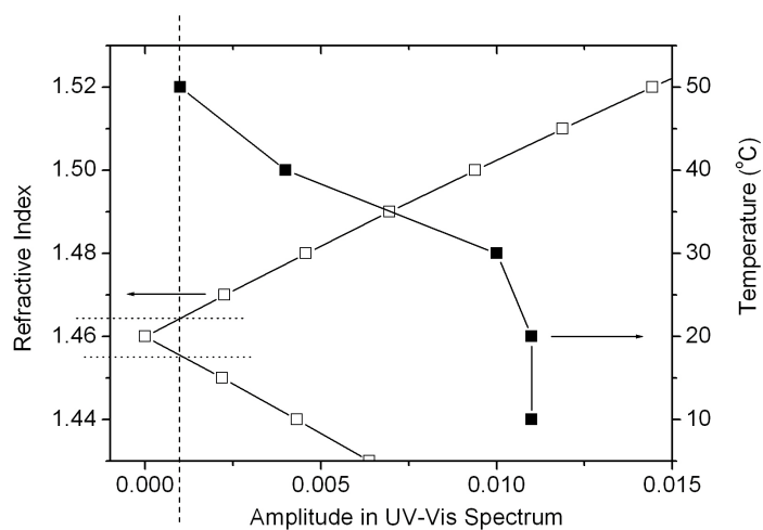
Figure S1 Relationships among amplitude of Fabry-Pérot fringes, refractive index and fabrication temperature. (Solid Square: read from UV-visible spectra; Void Square: Calculate according to Equation (2))
