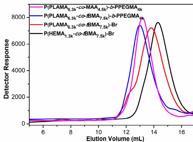
Fig. S1 GPC traces of P(HEMA 1.3k - co -tBMA 7.5k )-Br, P(PLAMA 6.3k - co -tBMA 7.5k )-Br, P(PLAMA 6.3k - co -tBMA 7.5k )- b -PPEGMA 4k , and P(PLAMA 6.3k - co -MAA 4.5k )- b -PPEGMA 4k .
