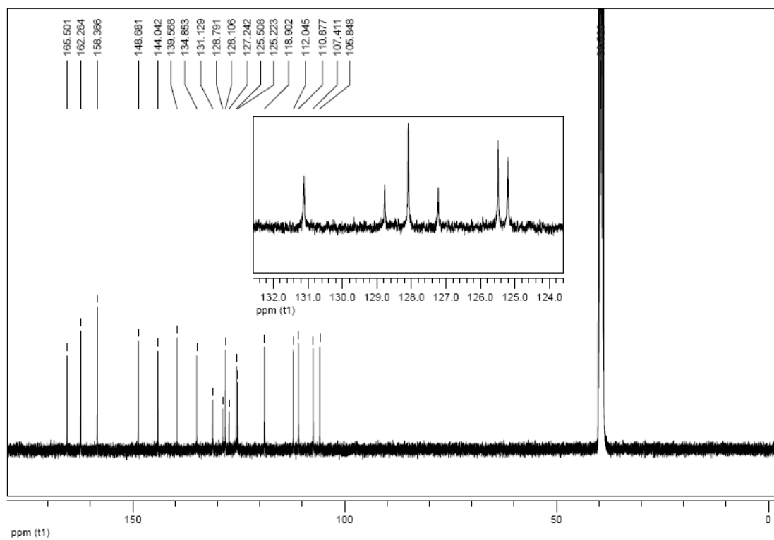
Fig. S2 13 C-NMR spectrum of BHPIA
