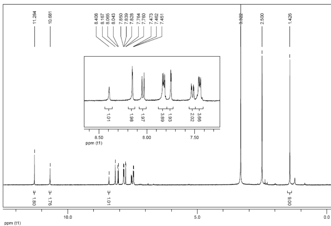
Fig. S3 1 H-NMR spectrum of BHPBIA
