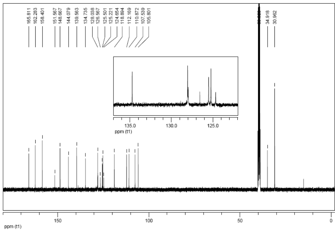
Fig. S4 13 C-NMR spectrum of BHPBIA
