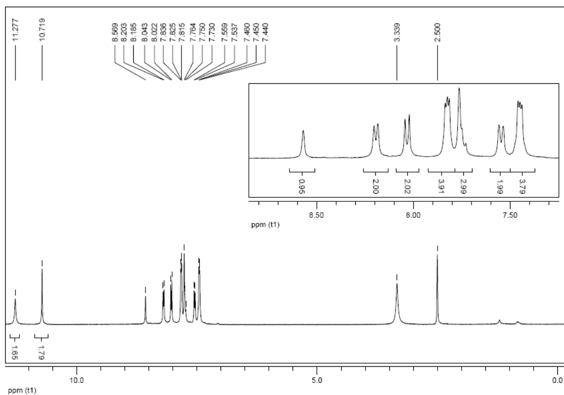
Fig. S1 1 H-NMR spectrum of BHPIA
