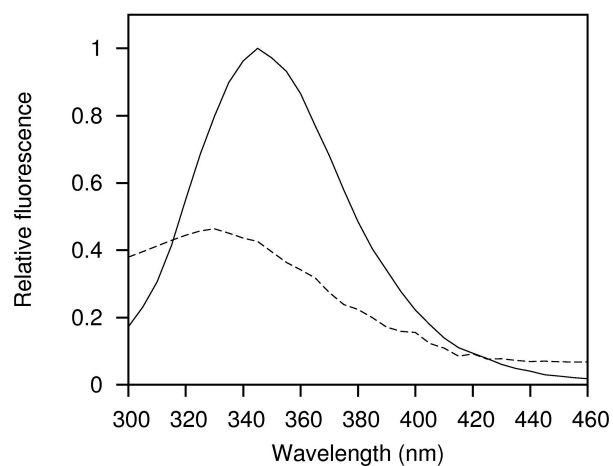
Figure S1. Tryptophan fluorescence emission spectra of BSA (0.1 mg/ml, pH 7.4). The figure shows the spectra of BSA before (solid line) and after (dashed line) 1 h shear treatment at 300 s -1 .
