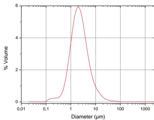
Fig. 1 Size distribution of primary particles measured by static light scattering measurements performed at 25 °C with a Mastersizer 2000 Hydro SM device (Malvern) . The samples were diluted in the measuring cell (simple scattering conditions) and submitted to a rather intense agitation to ensure homogeneity.
