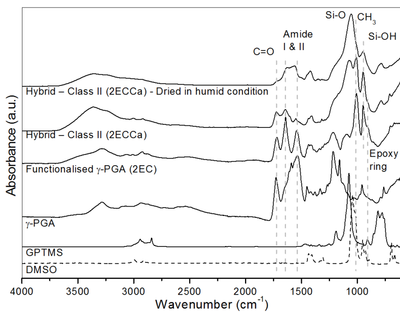
FTIR spectra of: DMSO; GPTMS; \gamma -PGA; functionalised \gamma -PGA (2EC); a class II silica (+ CaCl 2 ) / \gamma -PGA hybrid (2ECCa); and the same hybrid dried under humid conditions.
