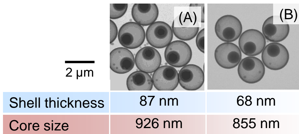
Figure S2 TEM images of rattle particles before (A) and after (B) the immersion to basic solution, respectively.
