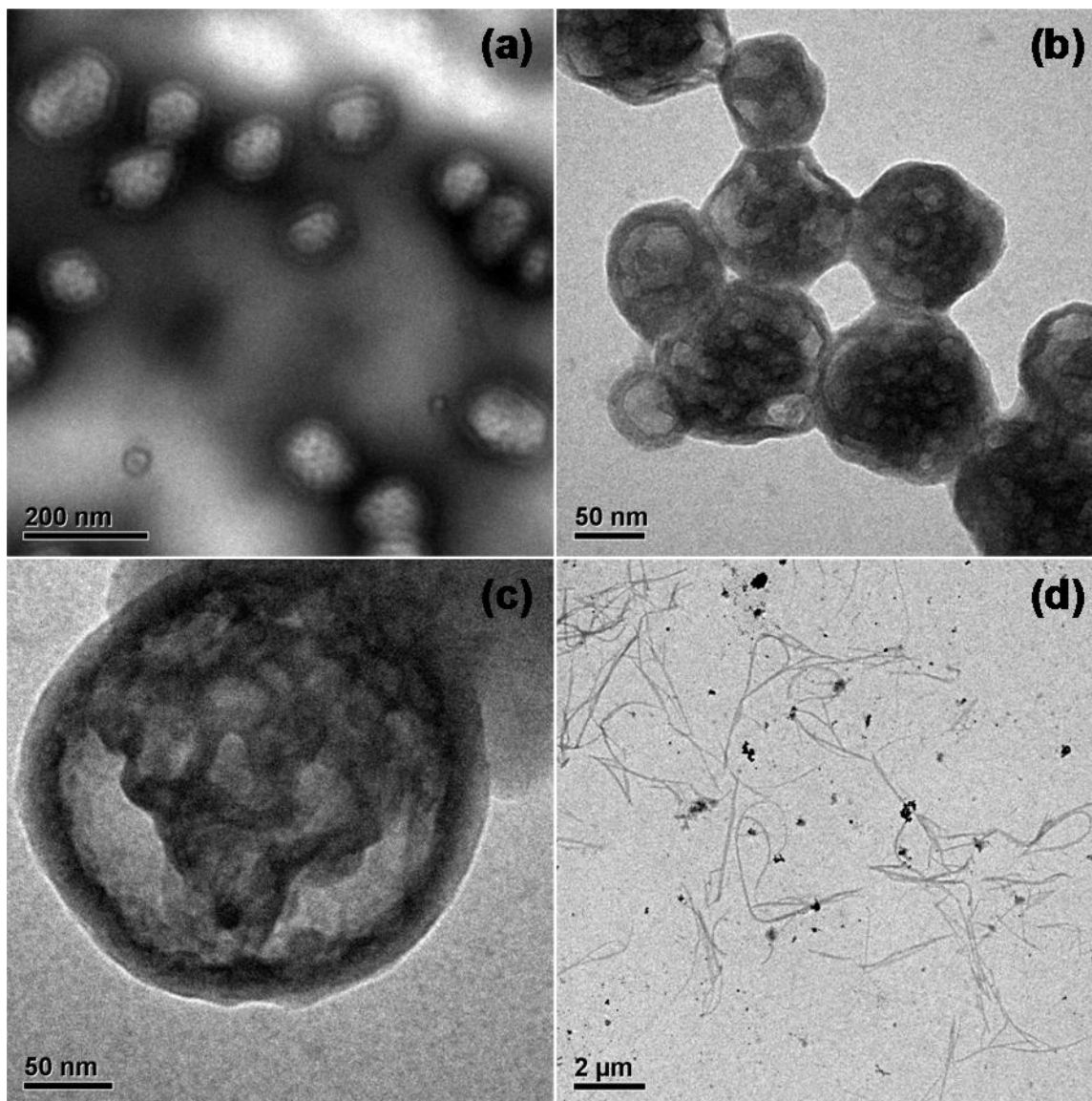
Figure S1. TEM images on the triblock hybrid at different temperatures. (a) 37 °C, stained with 1% PTA, scale bar 200 nm (b) 65 °C, unstained, scale bar 50 nm (c) 75 °C, unstained, scale bar 50 nm (d) 75 °C, unstained, scale bar 2 μm.
