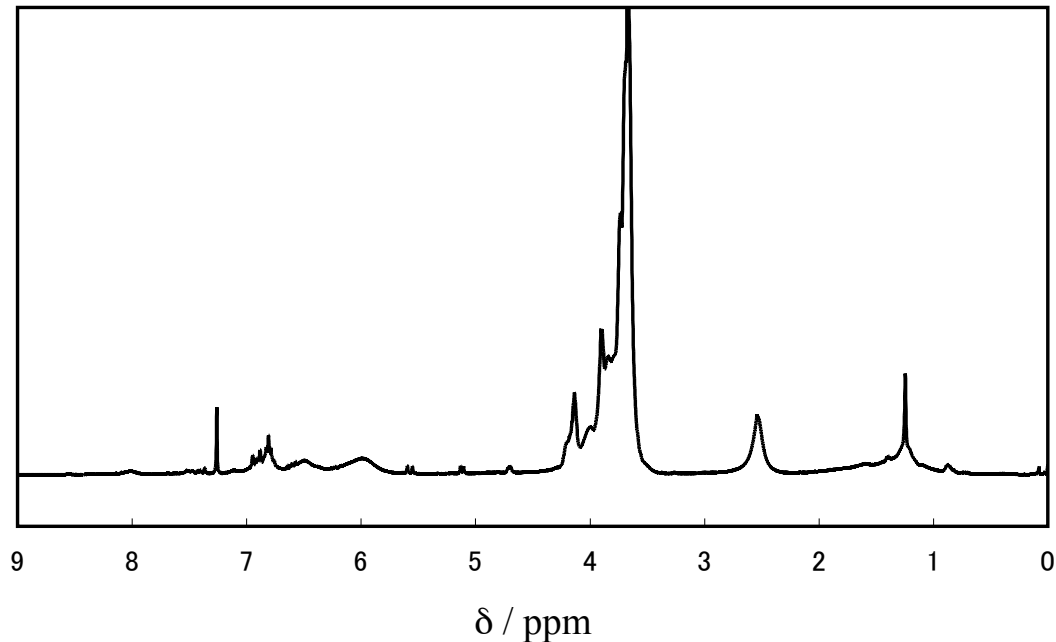
Figure S1. ^1\text{H-NMR} spectrum of poly(BC-co-cSP) in \text{CDCl}_3 .
