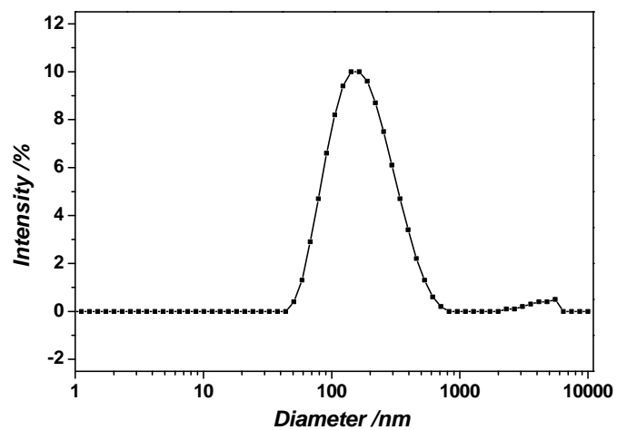
Fig. 1. Particle Size Distribution in „low water“ solvent.
