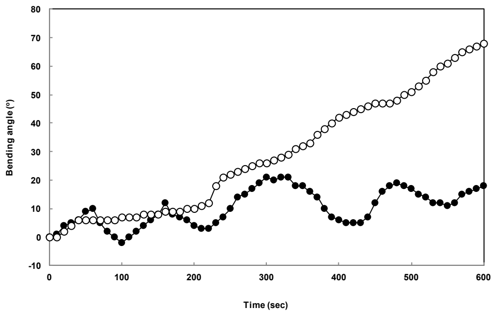
Fig. S1 The reversible bending and straightening behaviors of 1.0 (closed circle) and 0.1 mM (open circle) NBA-loaded palm-shape bilayer gels consisting of polyacid P(NIPAAm- co -CIPAAm) and polybase P(NIPAAm- co -DMAPAAm) layers with respect to time.
