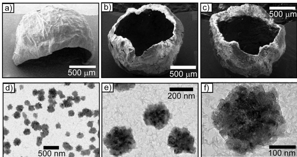
5 Fig. S1. a-c) SEM images of HSSP (level 3 structures) (PAA concentration = 7.7 mM). d-f) TEM images of HSSP (level 2 structures) (PAA concentration = 7.7 mM).
