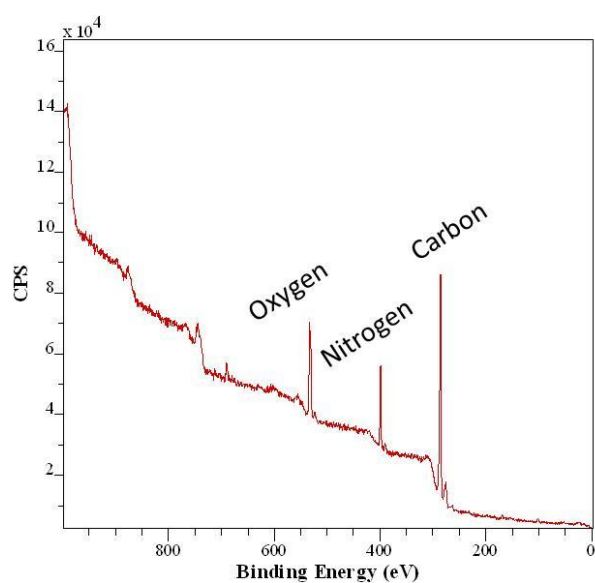
Figure S1. Typical XPS survey spectrum of an AApp coating
