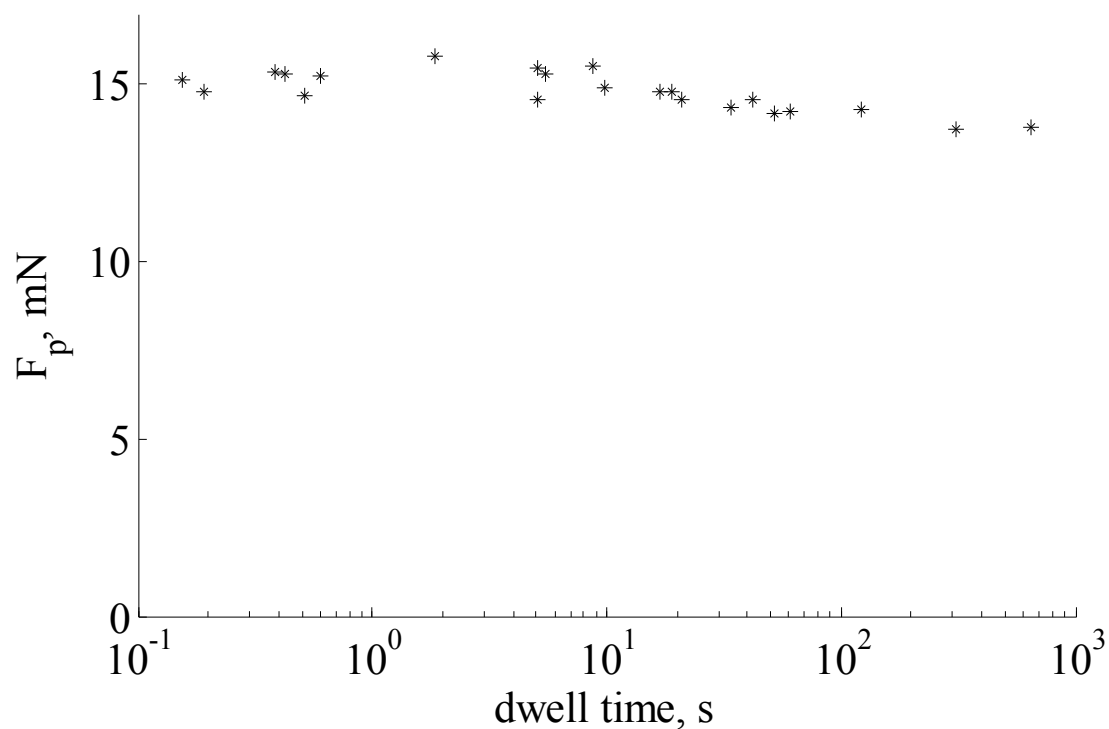
Figure S1. Dependence of pull-off force on the dwell time between loading and unloading for smooth sample on smooth substrate in presence of oil.
