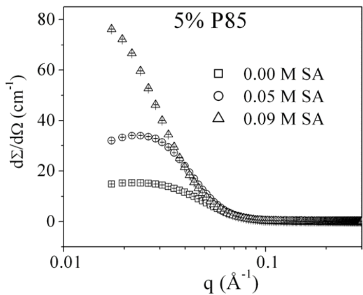
Figure B: SANS data of 5% aqueous P85 solutions at 30°C as a function of salicylic acid concentration along with their error bars.
