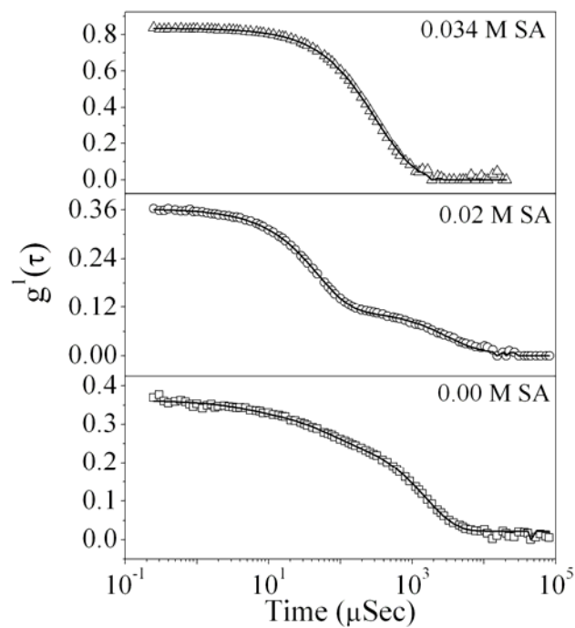
Figure A: Correlation function diagram of 1% P85 solution recorded at 30°C and at 130° scattering angle as a function salicylic acid (SA) concentration. The solid lines represent fit to the data based on CONTIN analysis.
