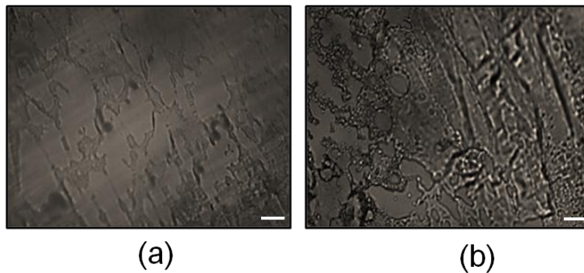
S1: Optical microscopy images of PS-LCE bilayer system showing (a) cracking and (b) delamination of the PS film at high strains.
