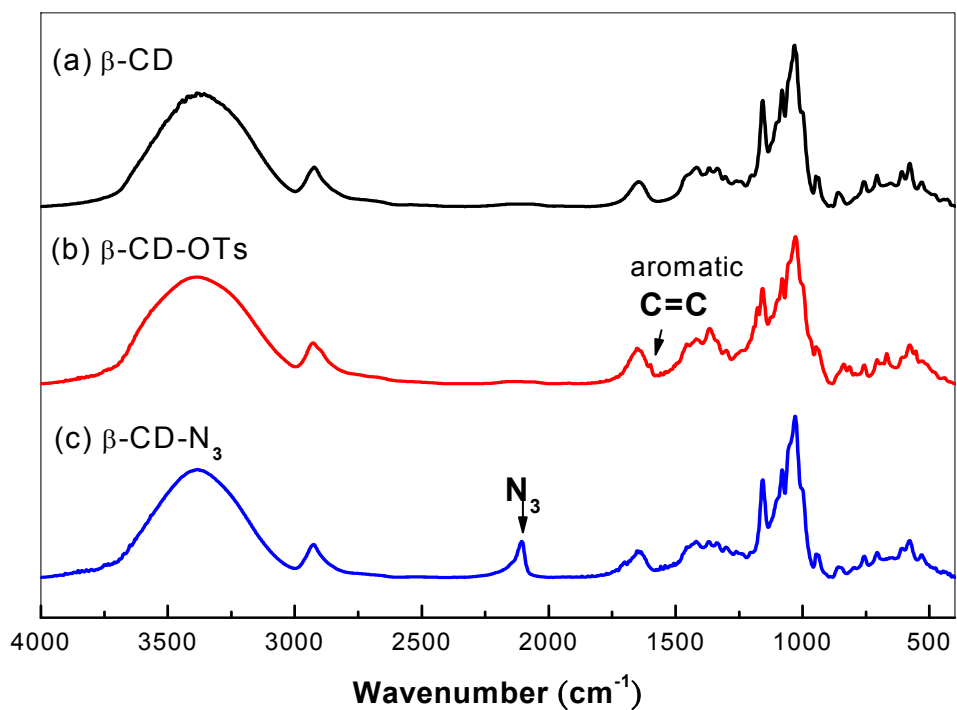
Figure S2: FT-IR spectra of (a) \beta -CD, (b) \beta -CD-OTs and (c) \beta -CD- \text{N}_3
