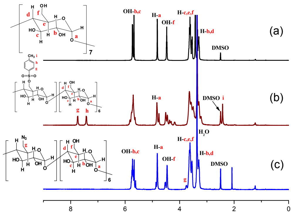
Figure S1: ^1\text{H} NMR spectra of (a) \beta -CD, (b) \beta -CD-OTs and (c) \beta -CD- \text{N}_3 (in d -DMSO).
