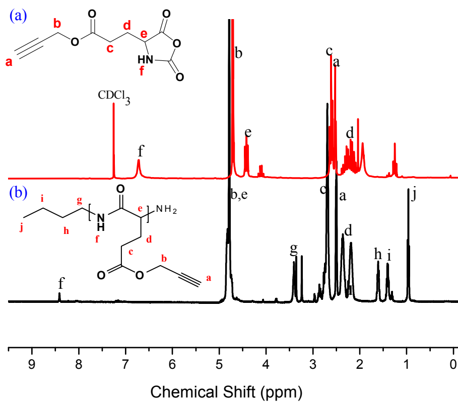
Figure S3: 1 H NMR spectra of (a) PLG-NCA (in d -CDCl 3 ) and (b) PPLG (in d -TFA).
