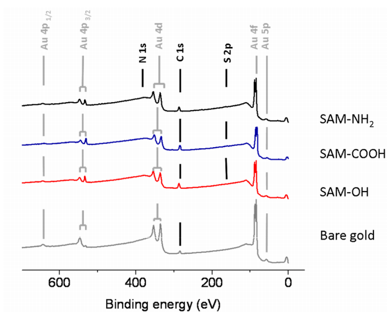
Figure 1. XPS spectra of bare Au, SAM-COOH, SAM-NH 2 and SAM-OH functionalized gold chips.
