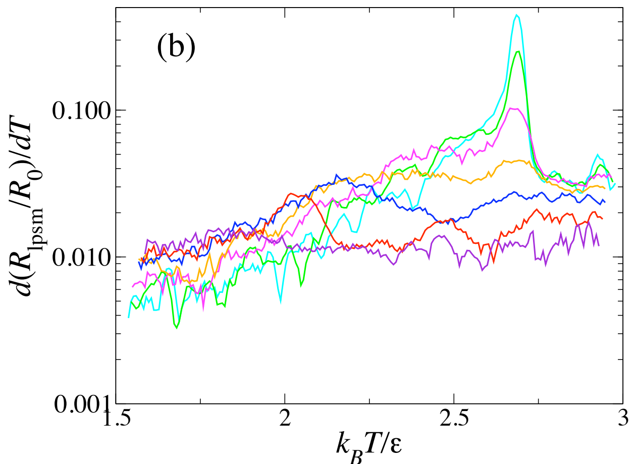
Caption: Temperature rate of Liposomes radius, vs. temperature. Curves from top to bottom at k_B T=2.6 correspond to liposomes composed of 80 000, 40 000, 20 000, 10 000, 5 000, 2 500, and 1 500 lipids, respectively.
