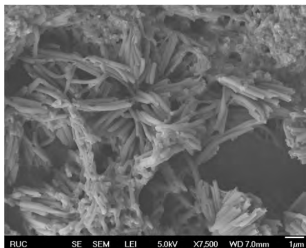
Figure S2. SEM image of RR-P3HT nanofibers obtained from the wetting of an AAO membrane with a P3HT/THF (20mg/ml) solution.
