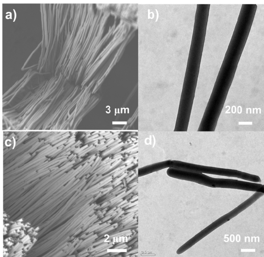
Figure S1. SEM and TEM images of PS nanofibers obtained from solvent annealing assisted wetting of AAO membranes: (a, b) PS annealed by the vapour of a \text{CCl}_4 /ethanol co-solvent (15 V% ethanol); (c, d) PS annealed by the vapour of a MEK/ethanol co-solvent (20 V% ethanol).
