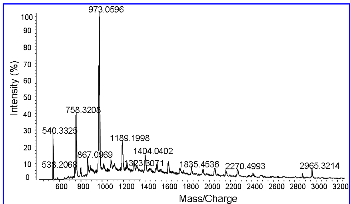
Figure S2. MALDI-TOF-MS spectrum of PMT14 using an AXIMA-CFR plus MALDI-TOF mass spectrometer.
