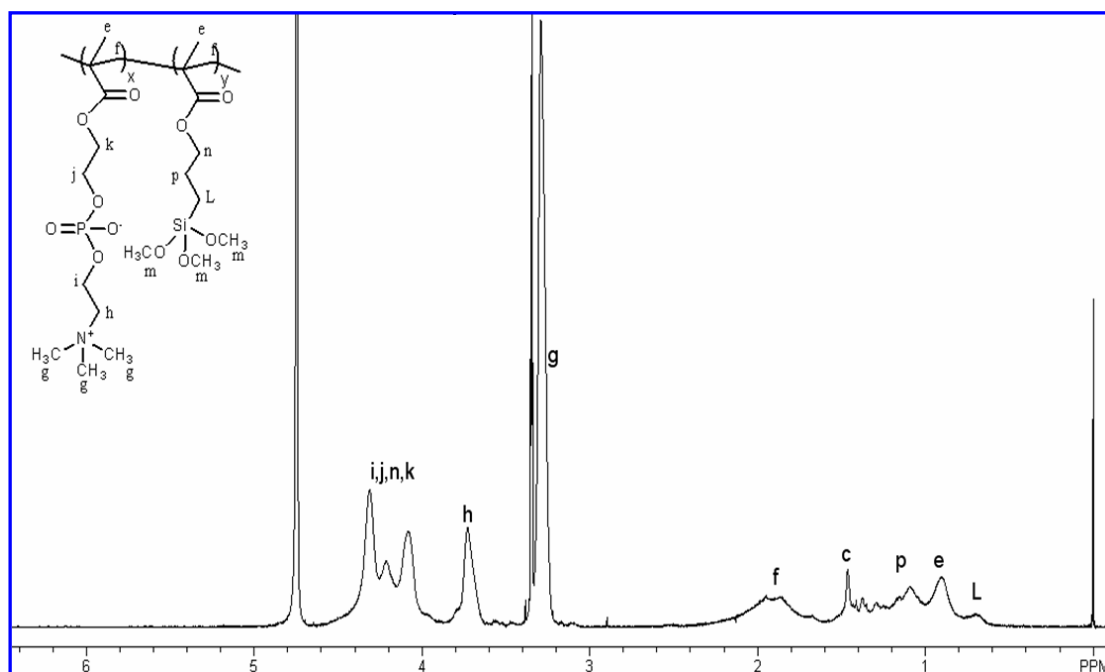
Figure S1. 1 H-NMR spectrum of PMT14 in D 2 O using an INOVA-400MHz NMR spectrometer
