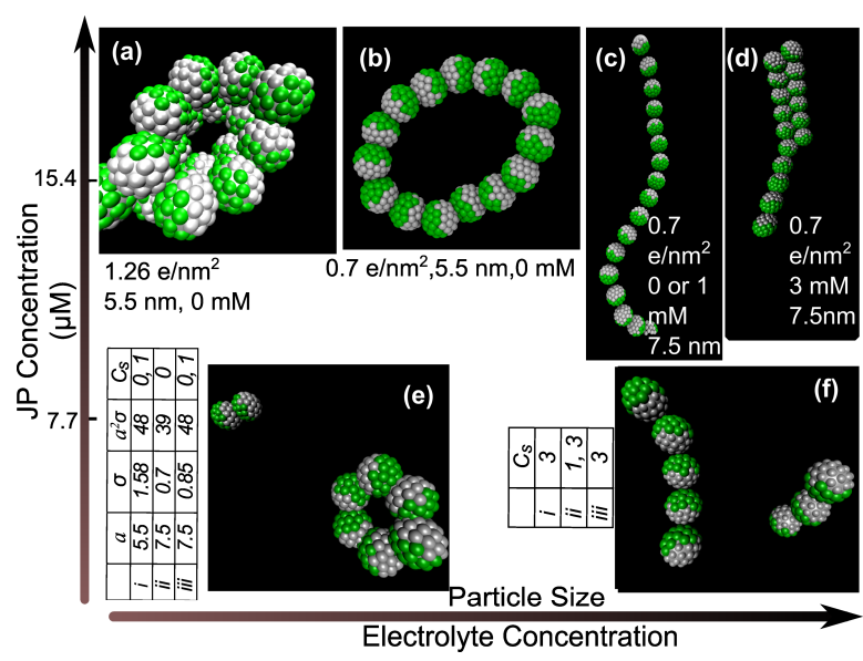
Cluster growth regimes at very low concentration region (no cluster-cluster interaction).
