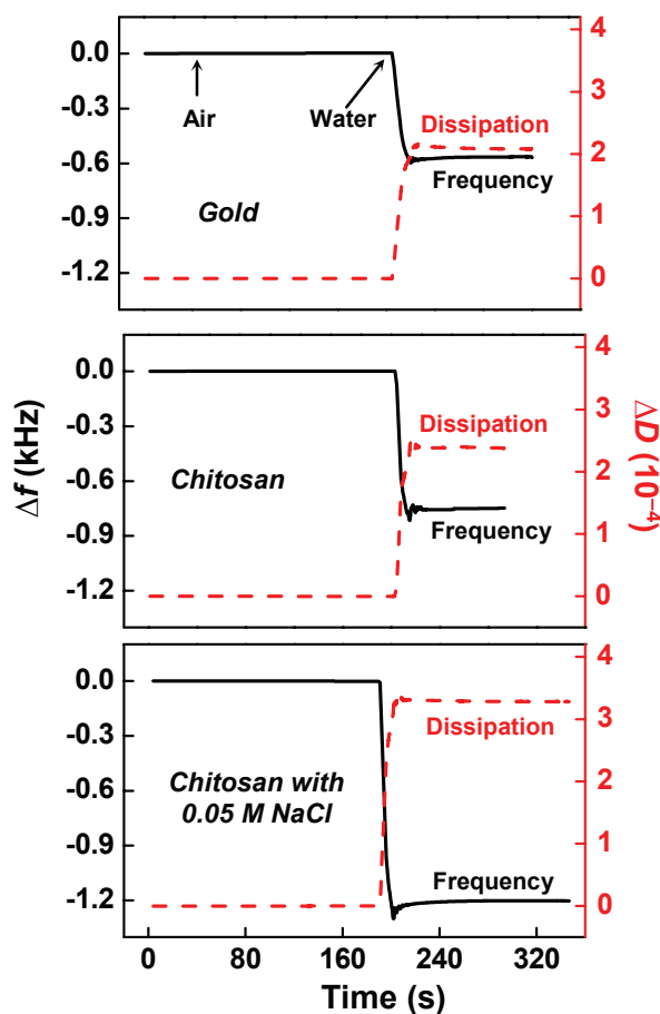
Fig. S1. Simultaneously measured \Delta f and \Delta D for bare gold QCM-D sensor (top), chitosan films electrodeposited in the absence (middle) and presence (bottom) of NaCl.
