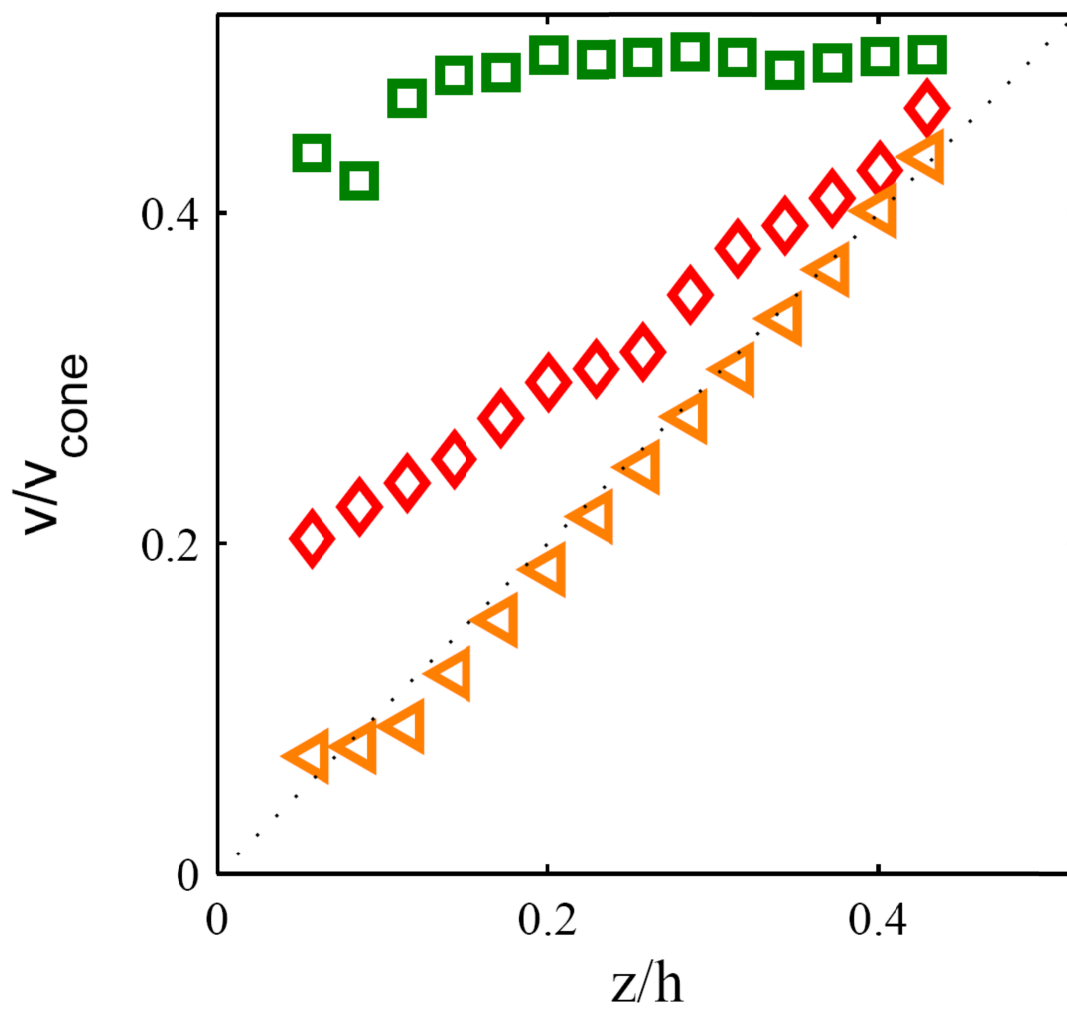
Supplementary Figure: Flow profiles from a colloid-polymer gel with 45% volume fraction, c/c^*=0.5 , at shear rates 0.1 1 and 10 1/s.
