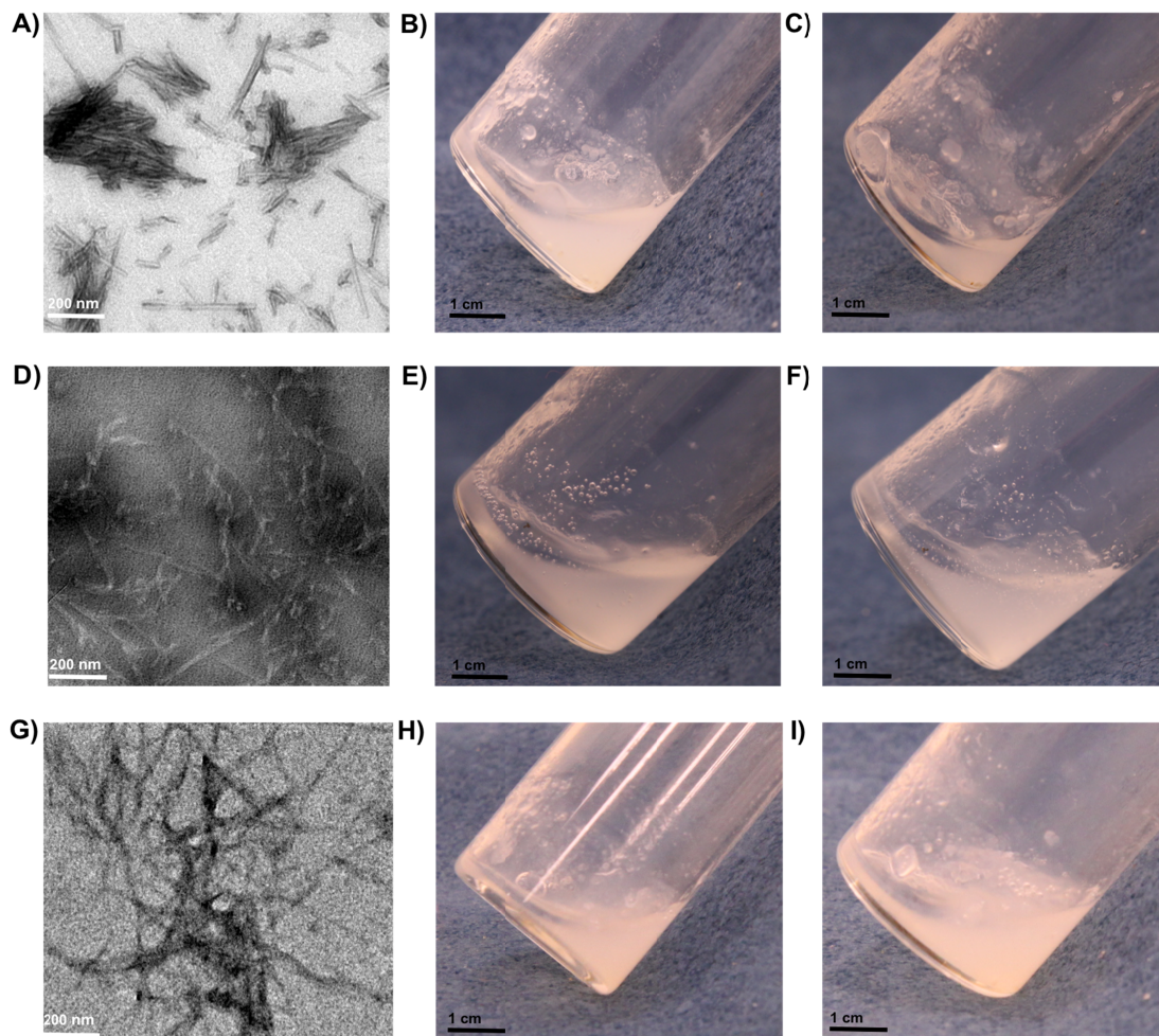
Supp. Fig. 1: IKVAV containing peptides that do not form a hydrogel at pH 7.4. A) TEM analysis of the disordered aggregates seen in the Fmoc-IKVAV system at pH 7.4 when formed using the pH switch. B) White aggregate suspension of Fmoc-IKVAV at 7.4. C) Similar aggregate observed when a temperature switch is applied. D, E, and F) Corresponding images of Fmoc-DIKVAV; G, H, and I) Corresponding images of Fmoc-DDDIKVAV.
