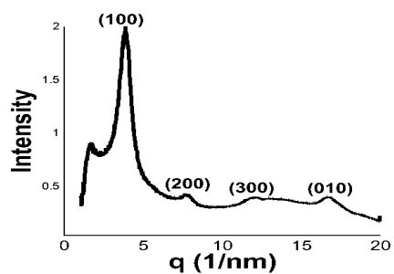
Fig. S1 Wide angle X-ray scattering (WAXS) of poly3-hexylthiophene (P3HT) film cast using chloroform. The plot shows clear molecular order with lamellar ( h00 ) peaks and p-p stacking (010) peak.
