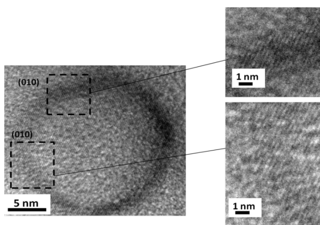
Fig. S2 Transmission electron microscopy (TEM) images of poly 3-hexylthiophene (P3HT) film showing \pi - \pi interchain stacking with sub-nanometer domain spacing.
