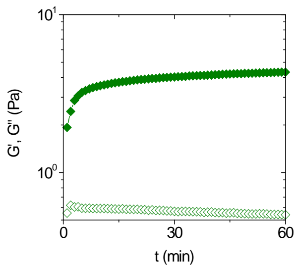
Fig. S1 Evolution of G' (closed symbols) and G'' (open symbols) during the assembly of 0.5 g/l K8/K18 at a frequency of 1 rad/s.
