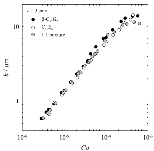
Figure A1: Thickness of the Frankel zone plotted versus the capillary number Ca of vertical foam films stabilized by \beta\text{-C}_{12}\text{G}_2 , \text{C}_{12}\text{E}_6 and their 1:1 mixture at c = 3 \text{ cmc} . The error bar is of the size of the symbols.
