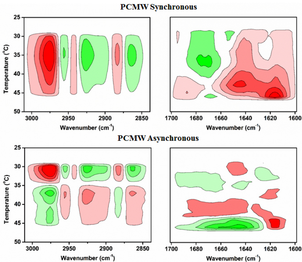
Fig. S2 PCMW synchronous and asynchronous spectra of [P 4,4,4,4 ][SS]-BSA-D 2 O solution between 25 and 50 °C during cooling. Red colors are defined as positive intensities, whereas green colors are defined as negative intensities.
