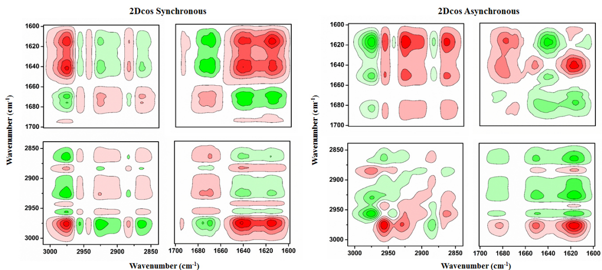
Fig. S3 2DCOS synchronous and asynchronous spectra of [P_{4,4,4,4}][SS] -BSA- D_2O solution during cooling between 25 and 50 °C. Red colors are defined as positive intensities, while green colors as negative ones.
