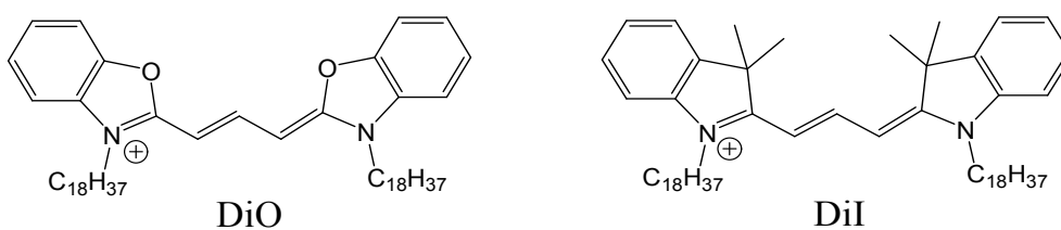
Scheme S1. Molecular Structures of DiO and DiI.
