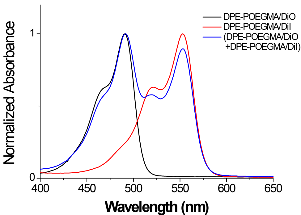
Figure S1. Absorption spectra of DiI/DiO in DPE-POEGMA aqueous solutions at room temperature.
