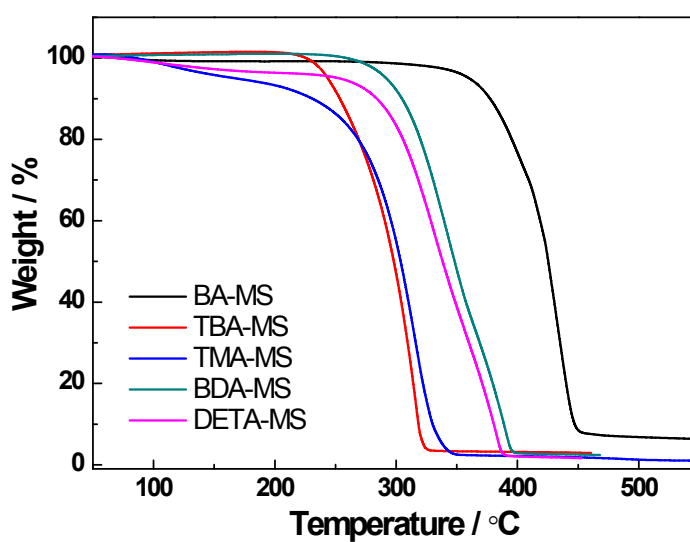
Figure S1. TGA curves for the pure PILs.
