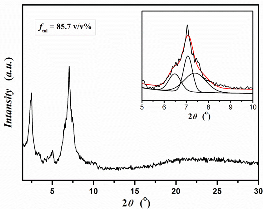
Fig. S1 XRD patterns of the xerogel samples of the organogels at f_{\text{tol}} = 100.0, 95.0, 90.0, 87.5 and 85.7 v/v%.
