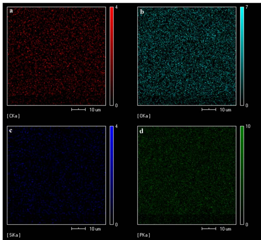
Fig.S2 The SEM-EDX maps showing distribution of C (a), O (b), Si (c) and P (d).
