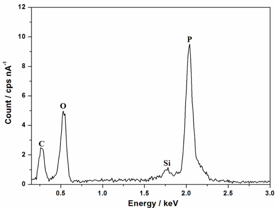
Fig.S1 The EDX spectrum of surface-sectional morphology for PA/SCPBI-1 membrane.
