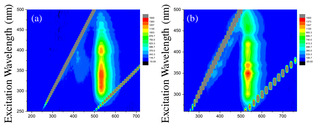
Fig. S2 Combined excitation-emission spectroscopy of (a) Ge NCs solution in dichloromethane (b) thin film of Ge NCs
