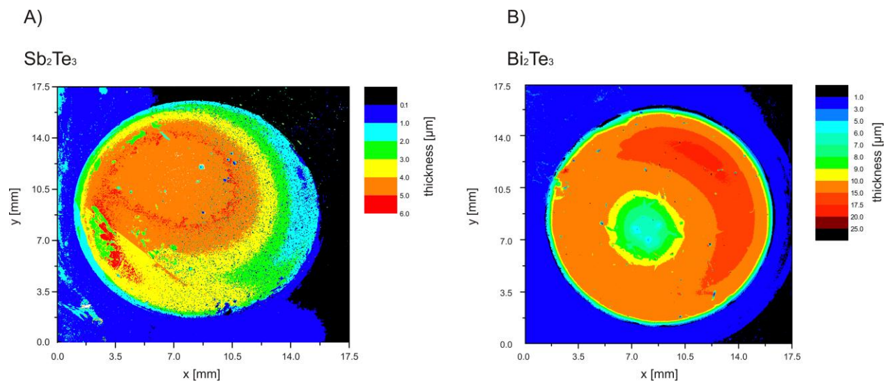
Figure S1: Optical profilometry thickness measurements for \text{Sb}_2\text{Te}_3 (A) and \text{Bi}_2\text{Te}_3 (B). The results confirm qualitatively the calculations from Au fluorescence intensities.
