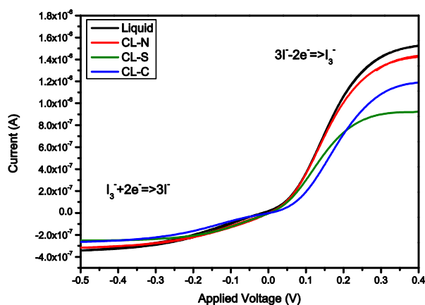
C-V curves of dummy liquid electrolyte and dummy gel electrolyte with different type of anionic hydrotalcite containing \text{I}_2 and PMII
