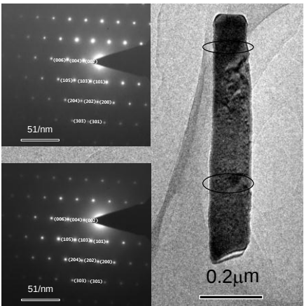
Figure S2 High-resolution transmission electron microscopy and the selected area electron diffraction patterns of a single TiO 2 nanorod.
