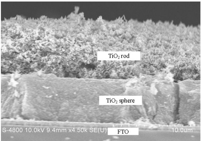
Figure S1 Cross-sectional image of bilayer structured TiO 2 film electrode.
