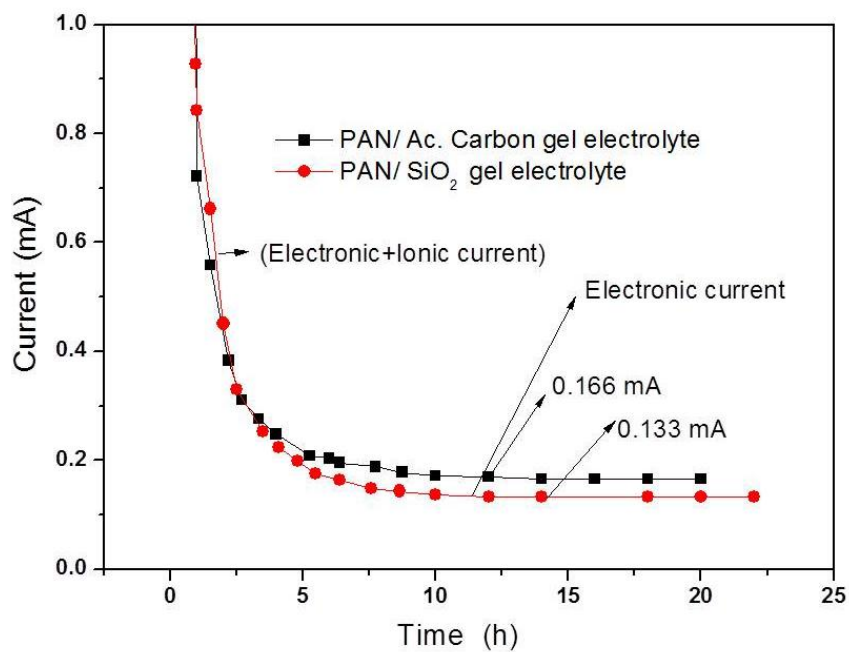
Figure S4. Determination of electronic current for PAN/ Ac.carbon and PAN/SiO 2 polymer gel electrolytes by Wagner's polarisation technique.
