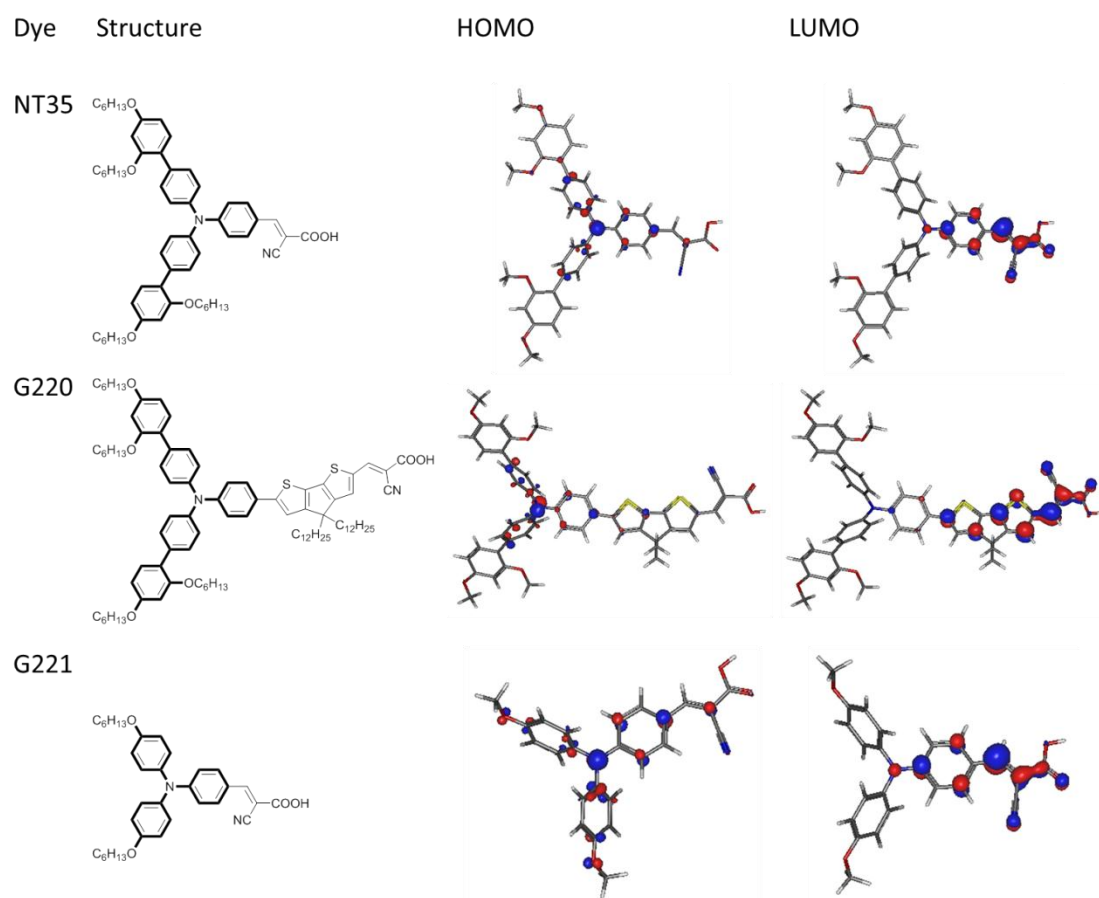
Figure S1. Density functional theory (DFT) at the M06/6-31G* level in an SMD (methylene chloride) solvation model
