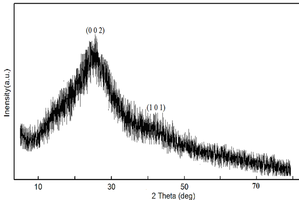
5 Fig. S1. XRD of the resulting graphitize carbon after composites of \text{H}_2\text{SO}_4 and \text{H}_2\text{O}_2 are hired to remove the \text{CeO}_2 .
