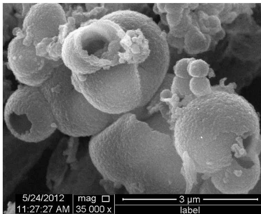
Fig. S2. SEM image of the resulting graphitize carbon after composites of \text{H}_2\text{SO}_4 and \text{H}_2\text{O}_2 are hired to remove the \text{CeO}_2 .
