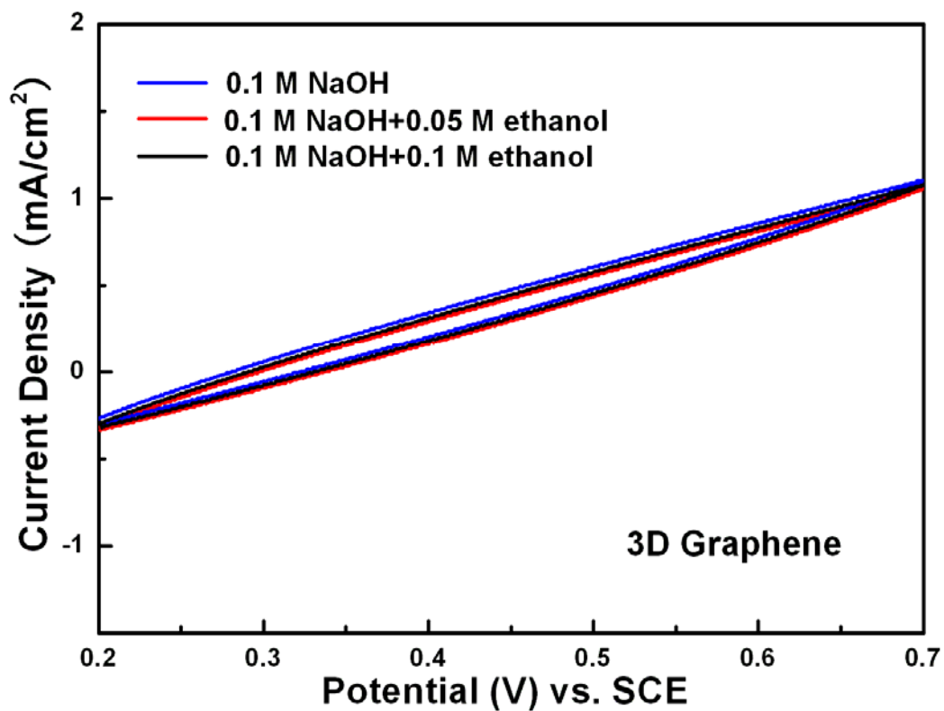
Figure S1. CVs of the pure graphene aerogel electrode in 0.1 M NaOH solution in the absence and presence of 0.05 M, 0.1 M ethanol. Scan rate: 0.1 V/s.
