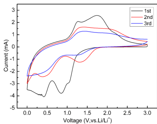
Fig. S2 CV curve of the rose-like \text{Co}_9\text{S}_8 electrode at 0.5 \text{ mV s}^{-1} scanning rate in the potential window from 0.01 V to 3.0 V (vs. Li + /Li).
