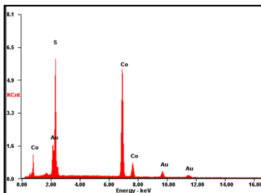
Fig. S1 Energy dispersive spectrum of the as-synthesized rose-like \text{Co}_9\text{S}_8 .
