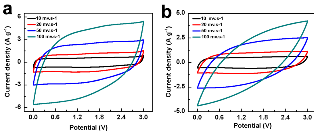
Fig. S3 CVs of a GAC 10 -based EC (a) and an AC-based EC (b) at different scan rates.
